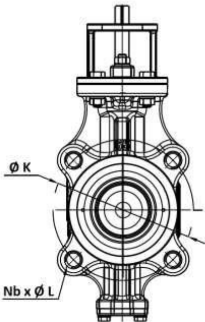
DN 50 – 65
